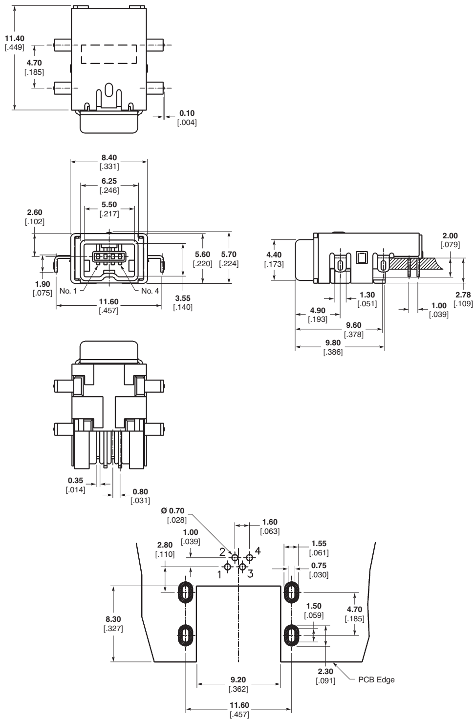
Recommended PCB Layout
