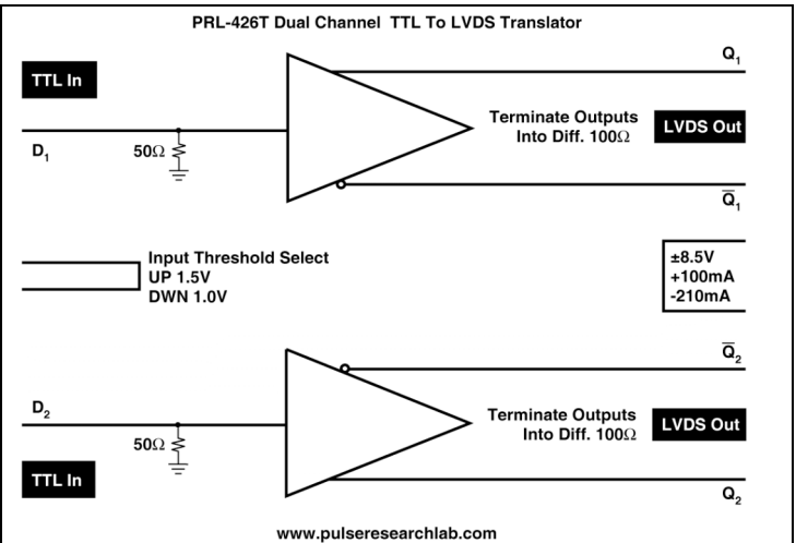
Fig. 2 PRL-426T Block Diagram
