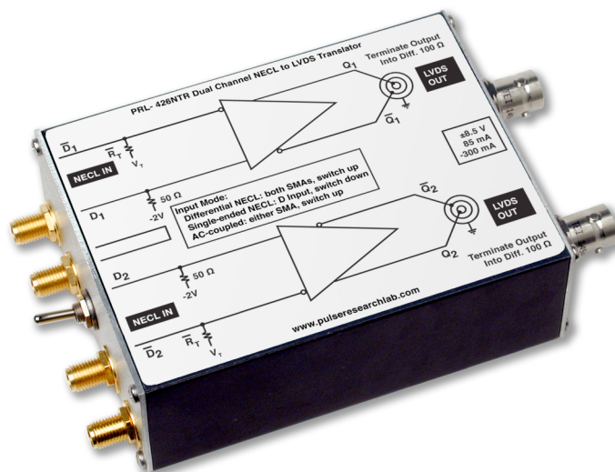
PRL-426NTR, NECL to LVDS (Triax) Translator
