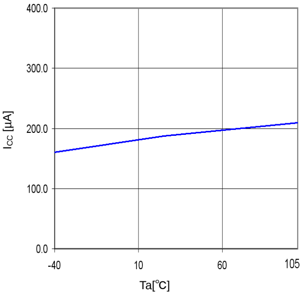
Figure 22. T_a - I_{CC}
