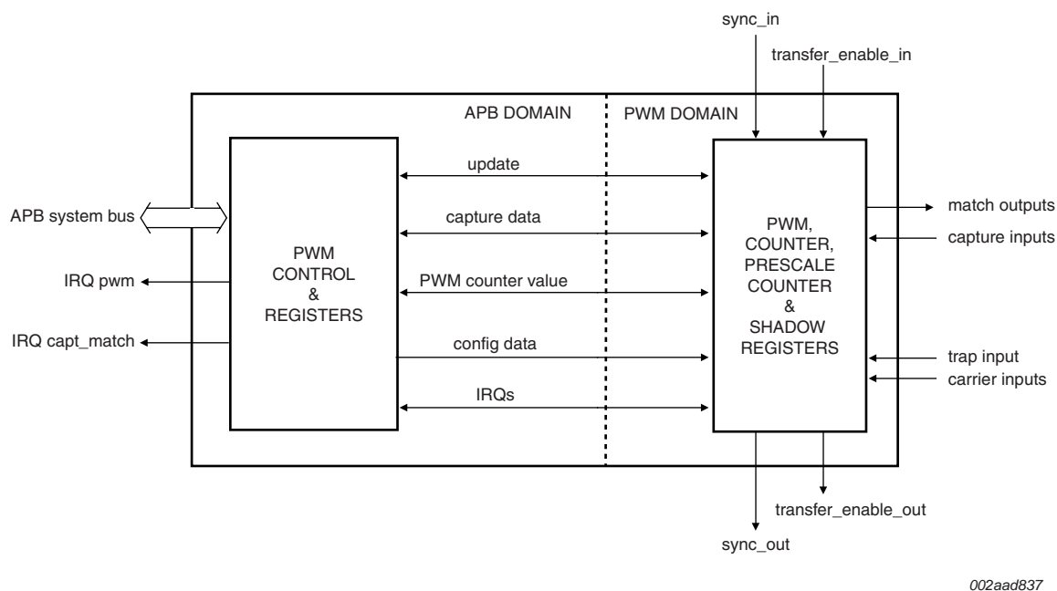
Fig 7. PWM block diagram
