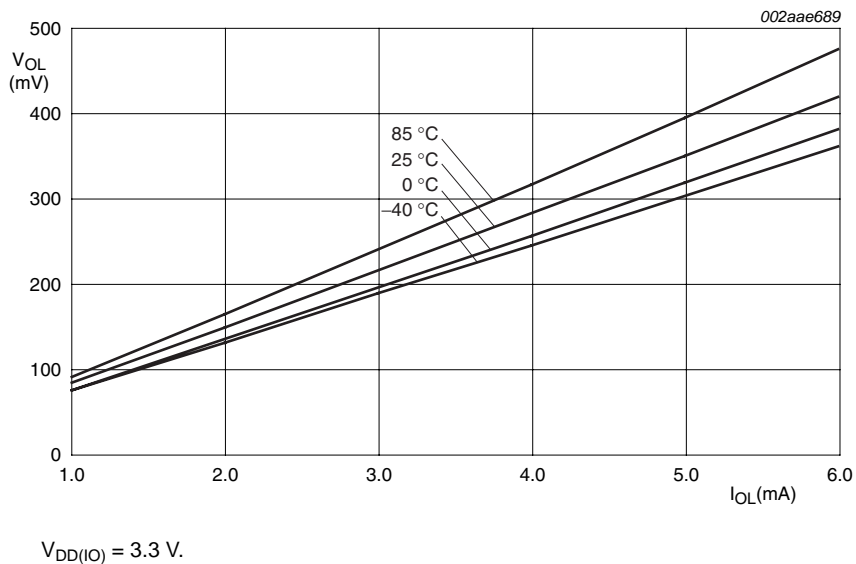
Fig 18. Typical LOW-level output voltage versus LOW-level output current
