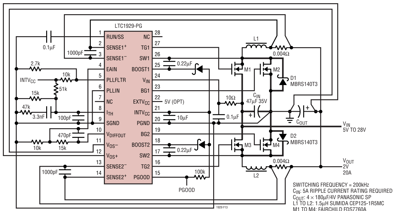
Figure 13. 2V/20A CPU Power Supply with Active Voltage Positioning
