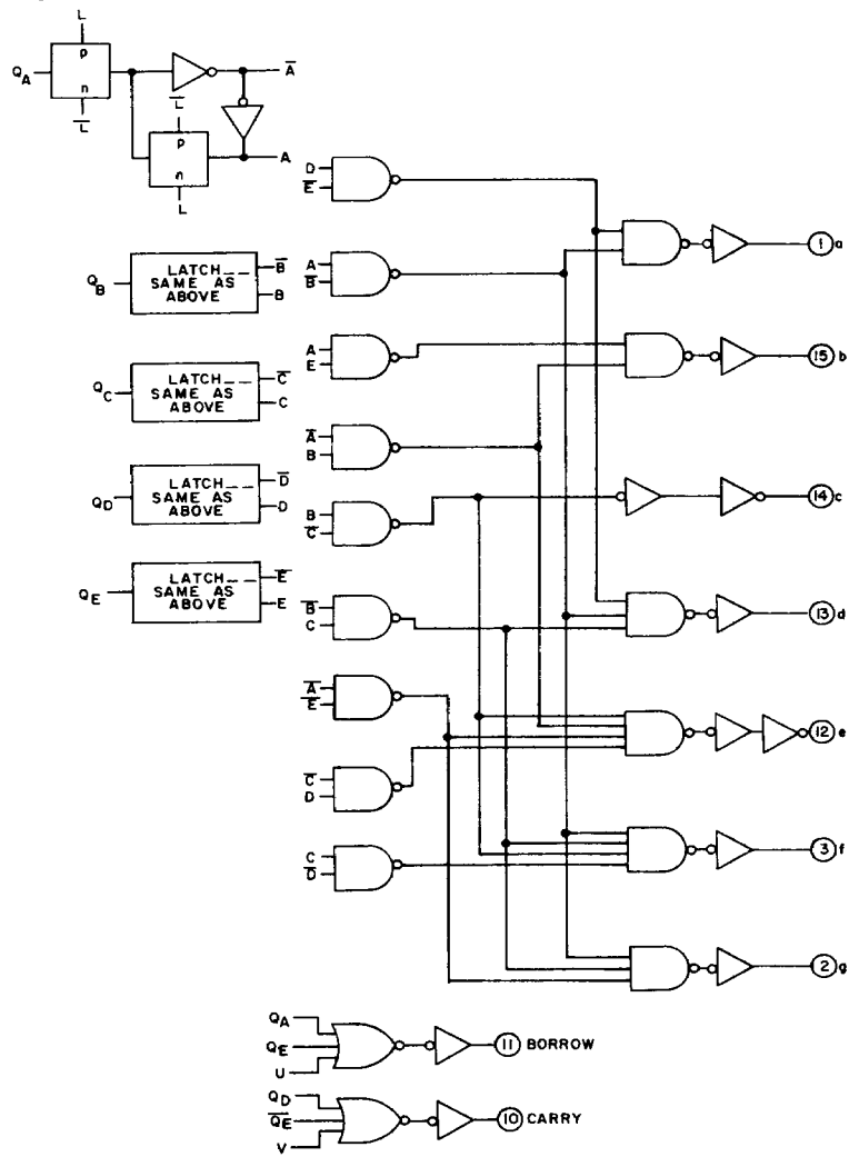
Fig. 2 - Logic diagram with flip-flop and output-driver details.
