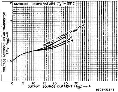
Fig. 9 - Voltage across bipolar transistor vs. output source current.
