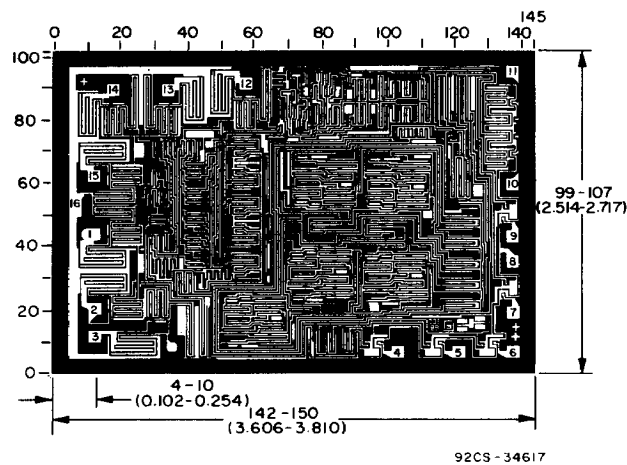
Dimensions and pad layout for CD40110B.
