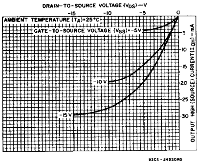
Fig. 5 - Typical carry or borrow output high (source) current characteristics.
