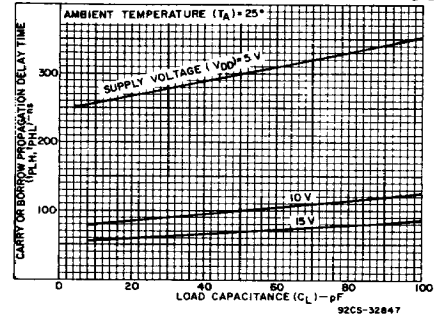
Fig. 8 - Typical carry or borrow propagation delay time vs. load capacitance.
