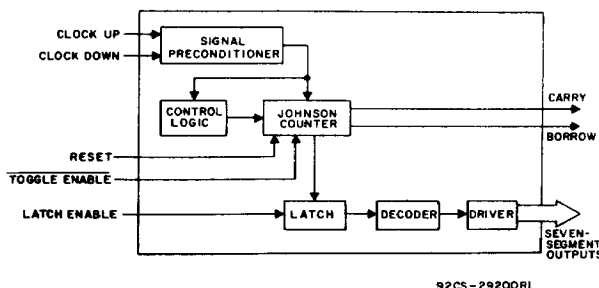
Fig. 1 - Functional diagram.
