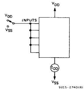
Fig. 12 - Quiescent device current.
