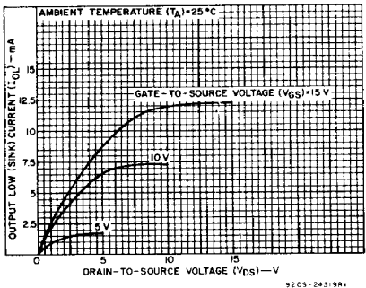
Fig. 4 - Minimum carry or borrow output low (sink) current characteristics.
