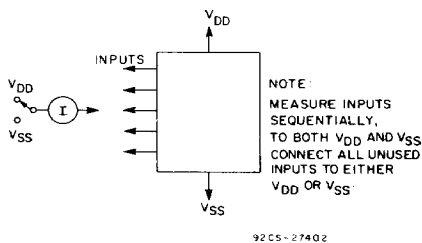
Fig. 13 - Input current.
