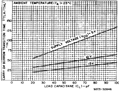
Fig. 7 - Typical carry or borrow transition time vs. load capacitance.
