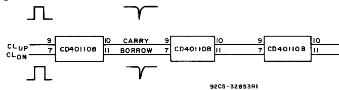
Fig. 15 - Cascading diagram.
