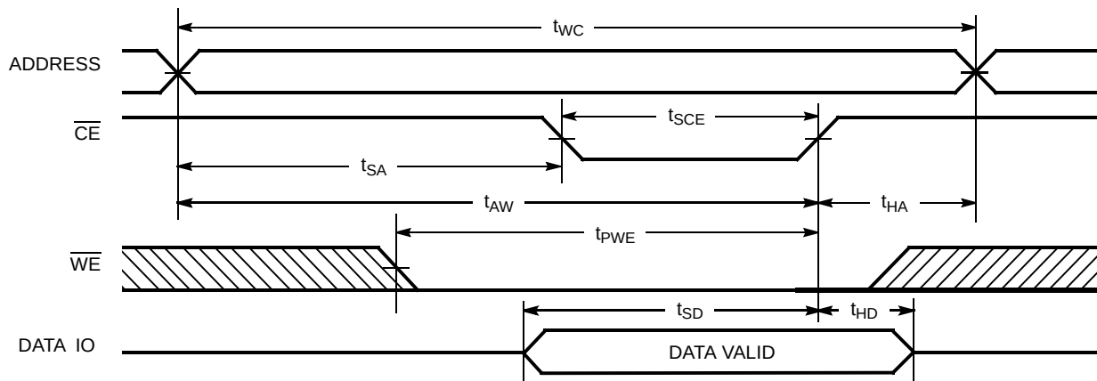
Figure 6. Write Cycle No. 2 ( \overline{\text{CE}} Controlled) [16, 17]
