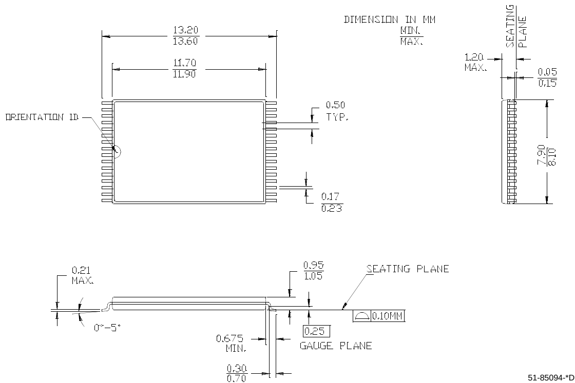
Figure 8. 32-Pin Shrunk Thin Small Outline Package (8 x 13.4 mm), 51-85094
