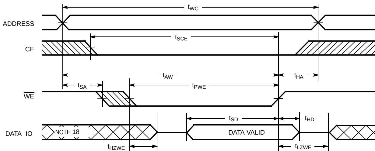
Figure 7. Write Cycle No. 3 ( \overline{\text{WE}} Controlled, \overline{\text{OE}} LOW) [17]
