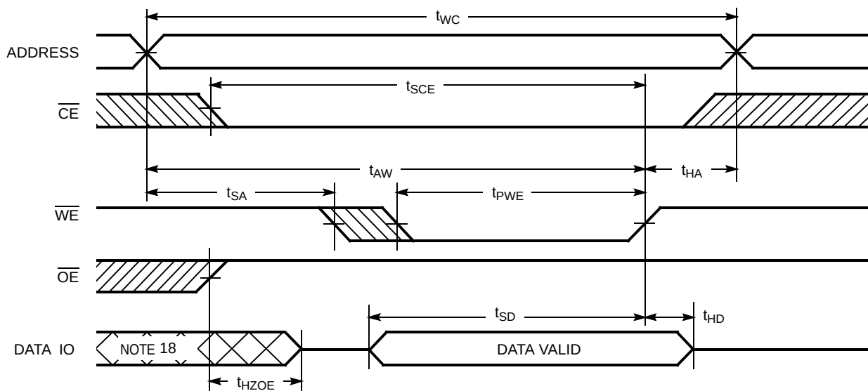
Figure 5. Write Cycle No. 1 ( \overline{\text{WE}} Controlled, \overline{\text{OE}} HIGH During Write) [16, 17]
