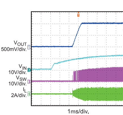
Start Up through VIN I_{OUT} = 0A
