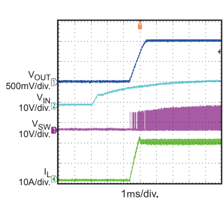
Start Up through VIN I_{OUT} = 20A
