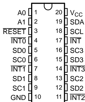
DGV, DW, OR PW PACKAGE (TOP VIEW)
