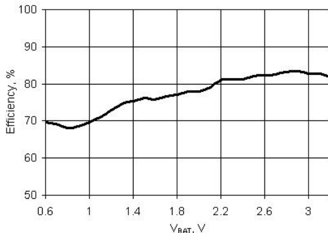
Figure 11-11. Efficiency vs V_{BAT}
