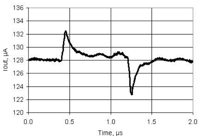
Figure 11-47. IDAC Glitch Response, Codes 0x7F - 0x80, 255 \mu A Mode, Source Mode, Fast Mode, V_{DDA} = 5 V
