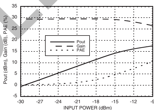
Power Compression @ 2200 MHz [2]
