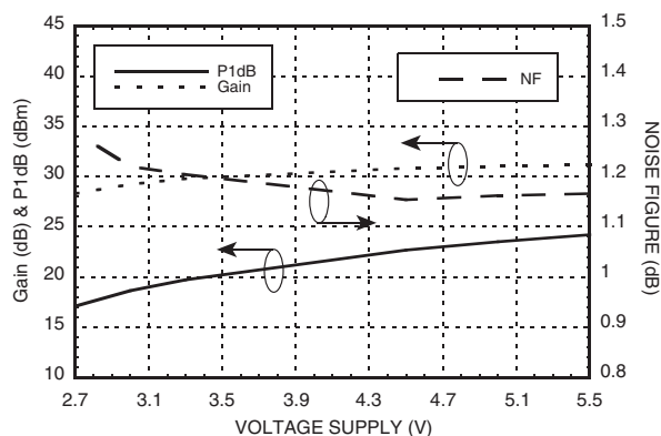
Gain, Power & Noise Figure vs. Supply Voltage @ 2200 MHz [3]
