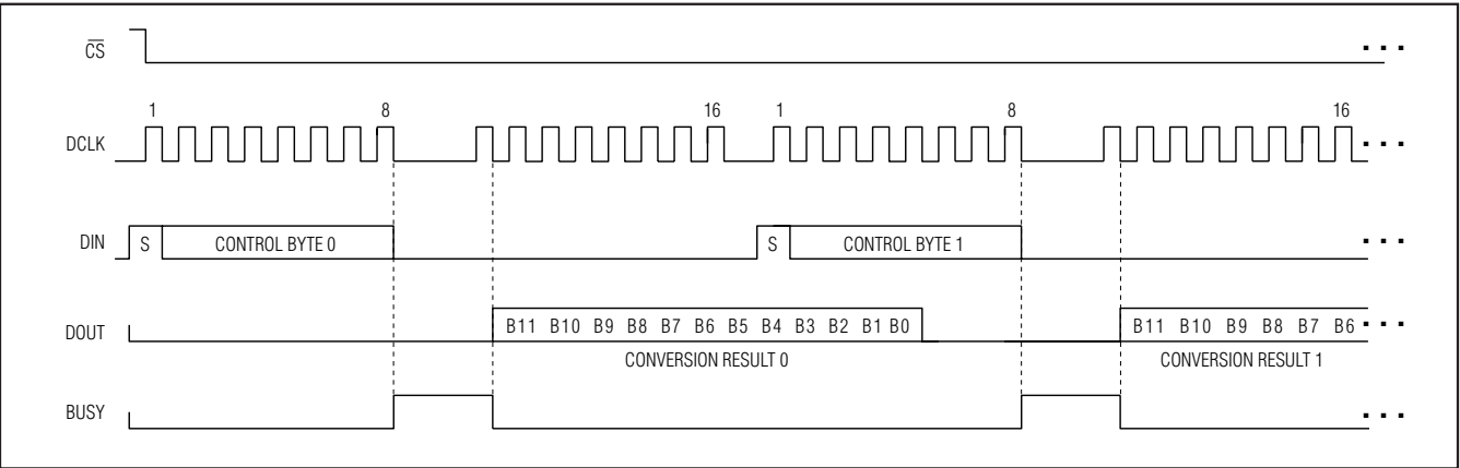
Figure 11. 16-Clock/Conversion Timing
