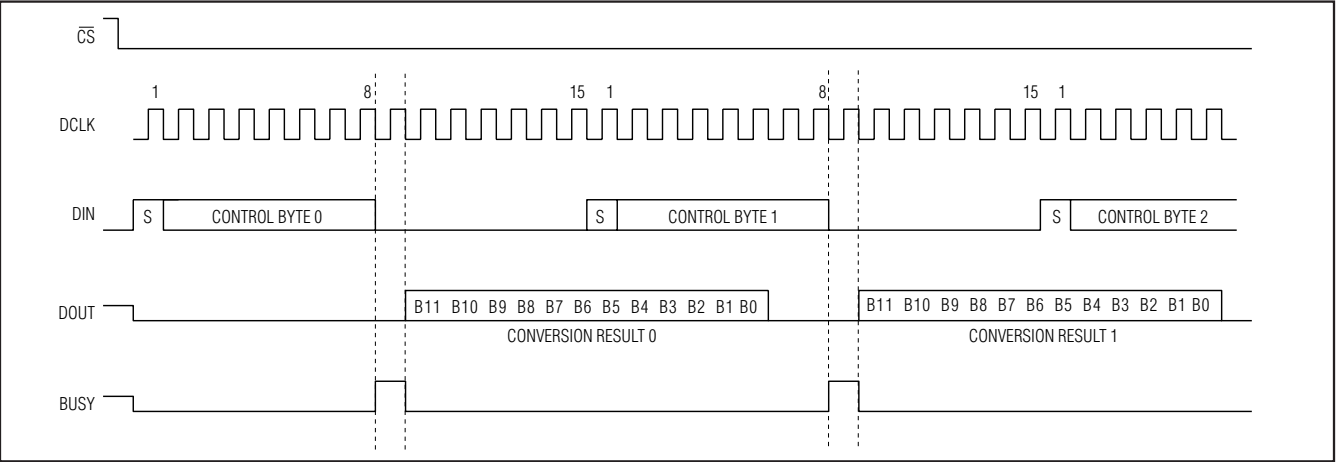
Figure 10. 15-Clock/Conversion Timing
