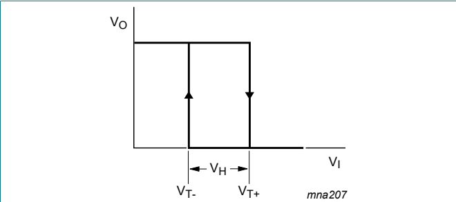
Fig. 12. Transfer characteristics
