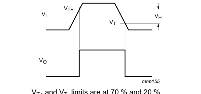
Fig. 15. Definition of V_{T+} , V_{T-} and V_H
