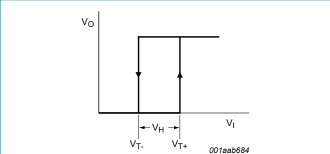
Fig. 14. Transfer characteristics
