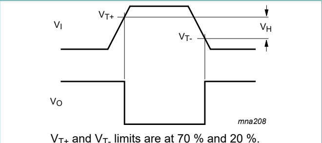
Fig. 13. Definition of V_{T+} , V_{T-} and V_H
