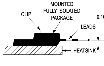
Figure 8. Clip Mounting Position for Isolation Test Number 2
