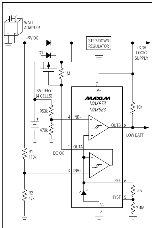
Figure 6. Battery Switchover Circuit
