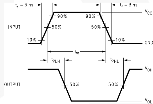
Figure 5. AC Waveforms
