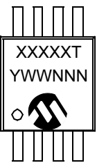
8-Lead MSOP
