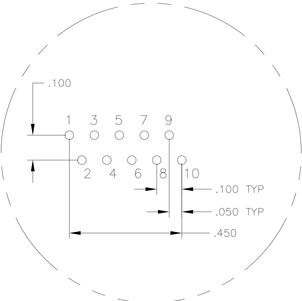
Pin Designations
