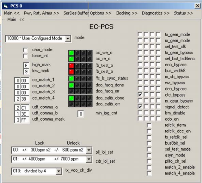
Figure 8-42. ORCAstra Main Window
