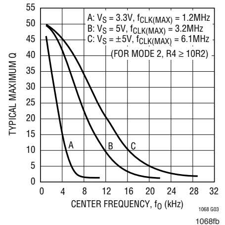
LTC1068-200 Maximum Q vs Center Frequency (Modes 1, 1b, 2)
