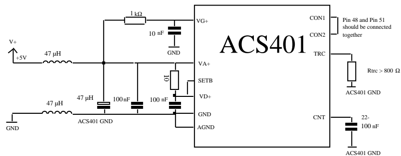
Figure 3. Recommended power supply layout
