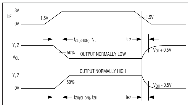
Figure 9. Driver Enable and Disable Times
