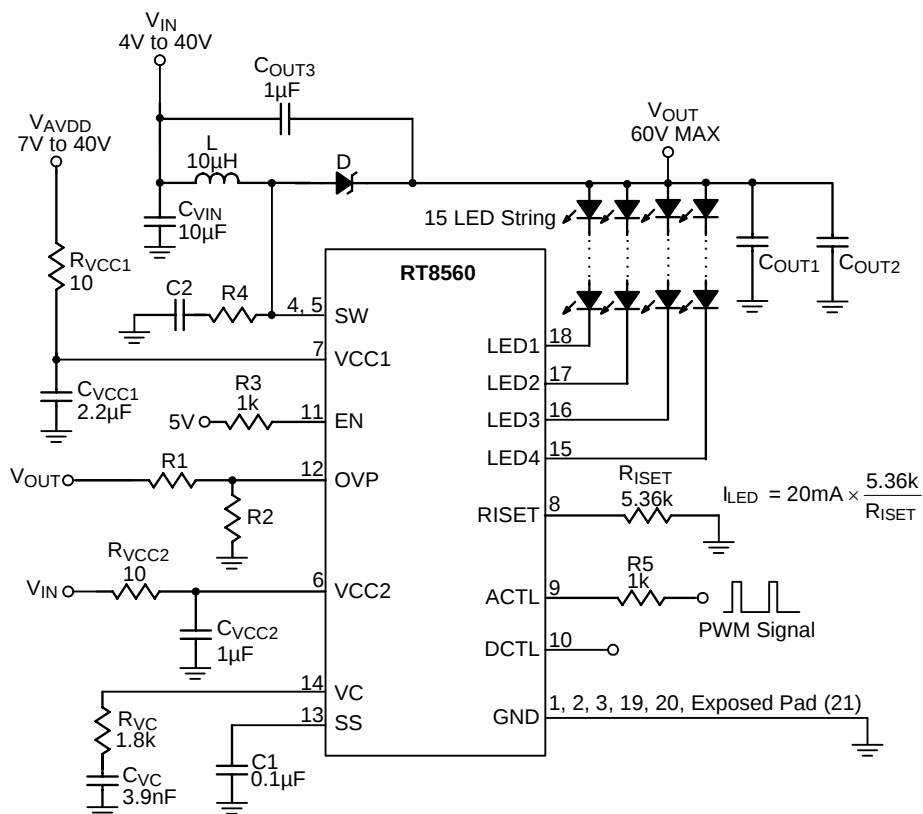
Figure 4. Wide Range VIN Application by Connecting VCC1 to LCD Driver Power AVDD
