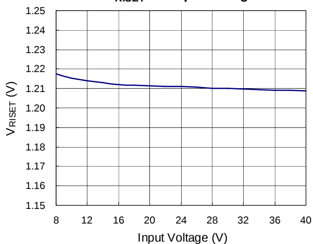
V_{RSET} vs. Input Voltage
