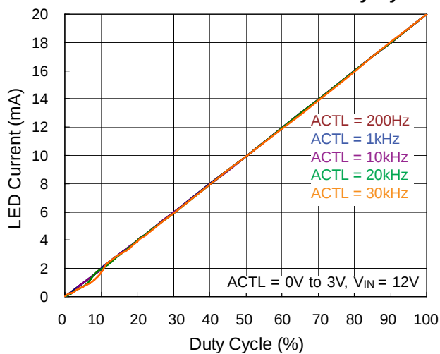
LED Current vs. ACTL PWM Duty Cycle
