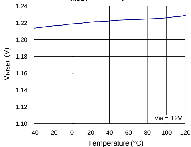
V_{RSET} vs. Temperature
