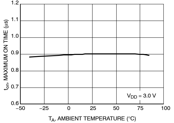
Figure 14. Maximum On Time versus Ambient Temperature
