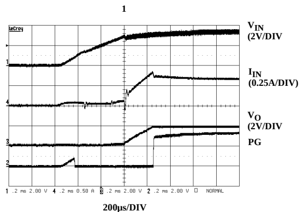
FIGURE 10. START-UP AT I_O = 600mA
