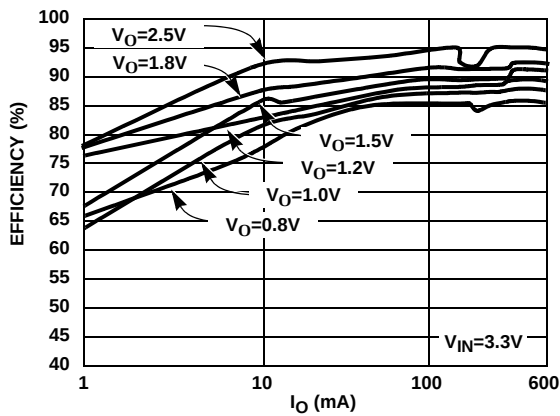
FIGURE 3. EFFICIENCY vs I_O (PFM/FWM MODE)
