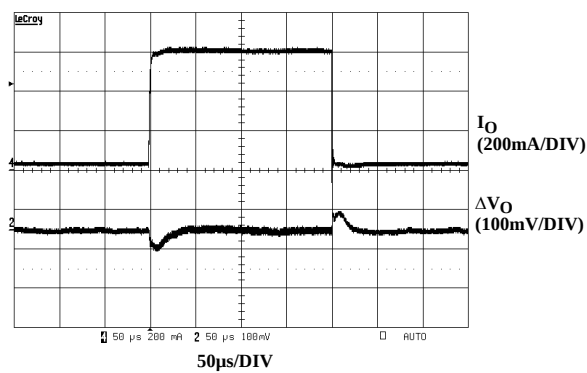
FIGURE 17. PWM LOAD TRANSIENT RESPONSE (30mA TO 600mA)
