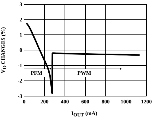
FIGURE 24. PFM-PWM LOAD REGULATION
