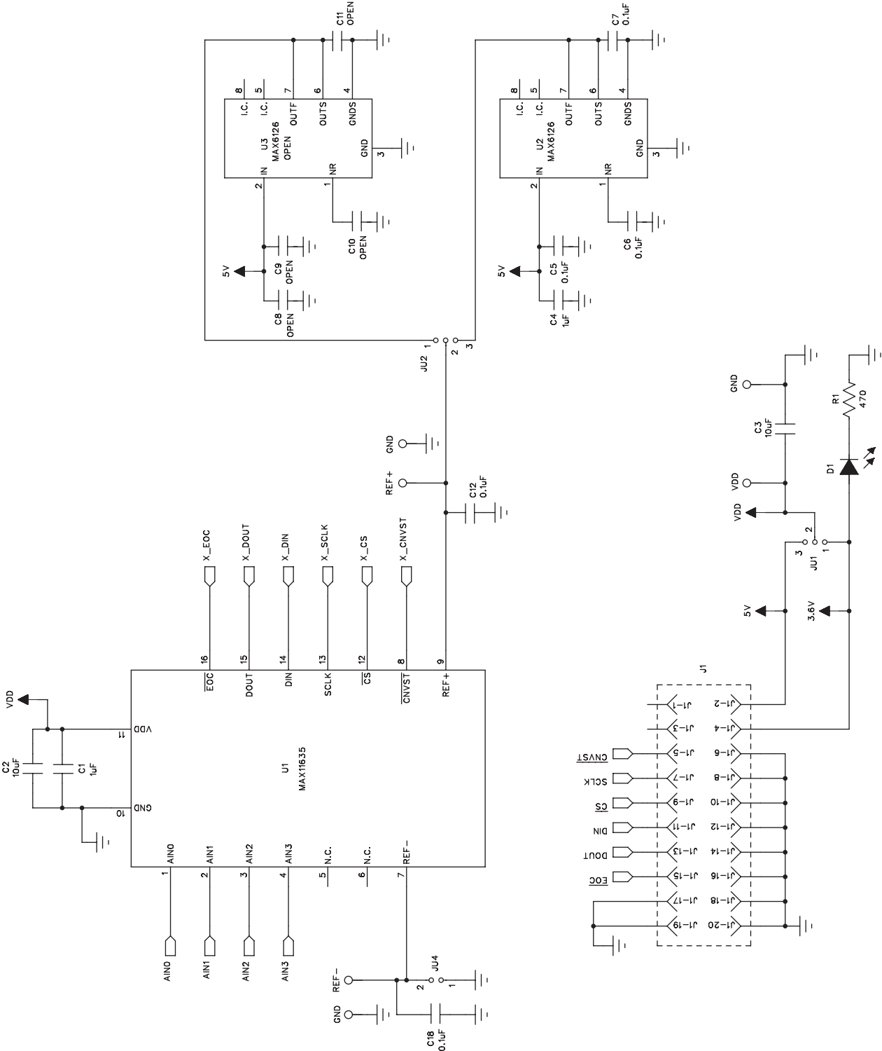
Figure 25a. MAX11635 Daughter Board Schematic (Sheet 1 of 2)
