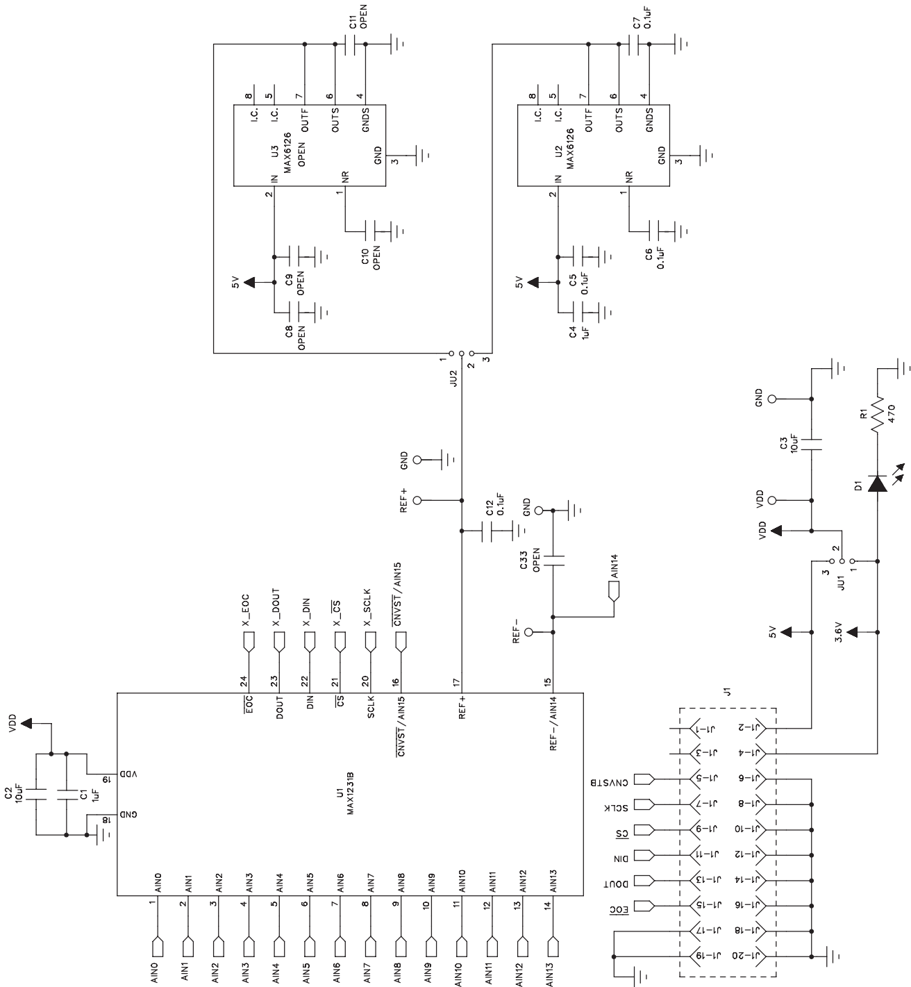
Figure 17a MAX1231B EV Kit Daughter Board Schematic (Sheet 1 of 3)
