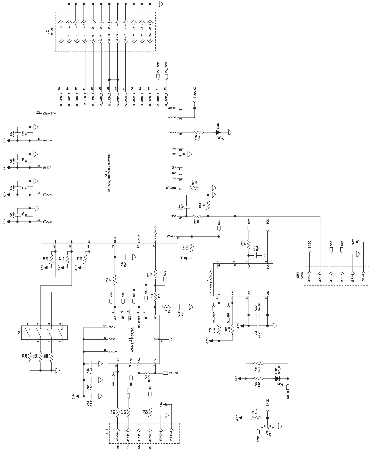
Figure 10b. MAX116XX SPI Master Board Schematic (Sheet 2 of 4)
