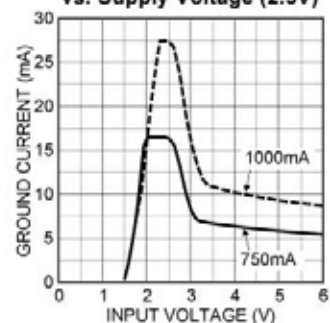
Ground Current vs. Supply Voltage (2.5V)
