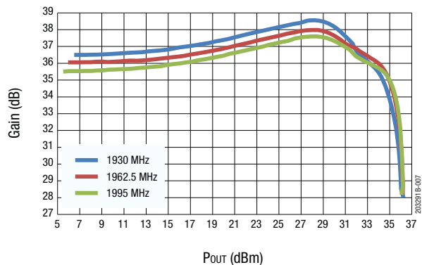
Figure 7. Gain vs P_{out} at Different Frequency
