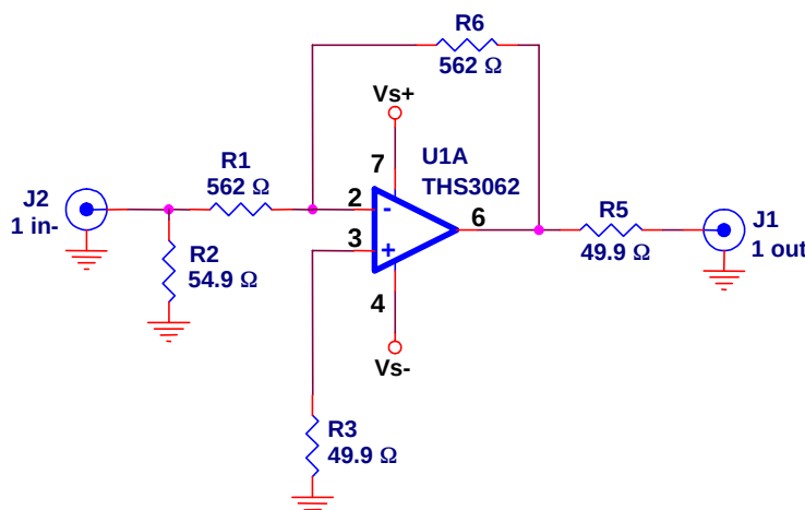
Figure 3-1. Inverting Gain Stage
