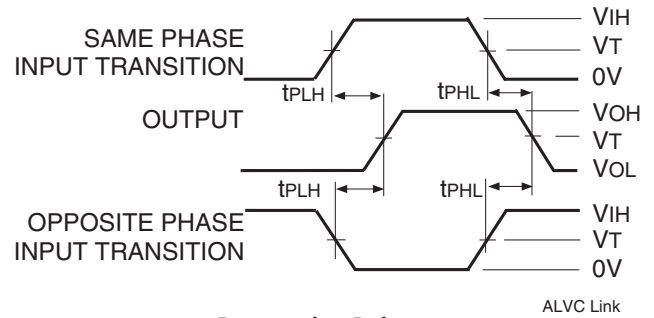
Propagation Delay
