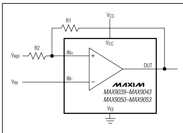
Figure 1. Additional Hysteresis
