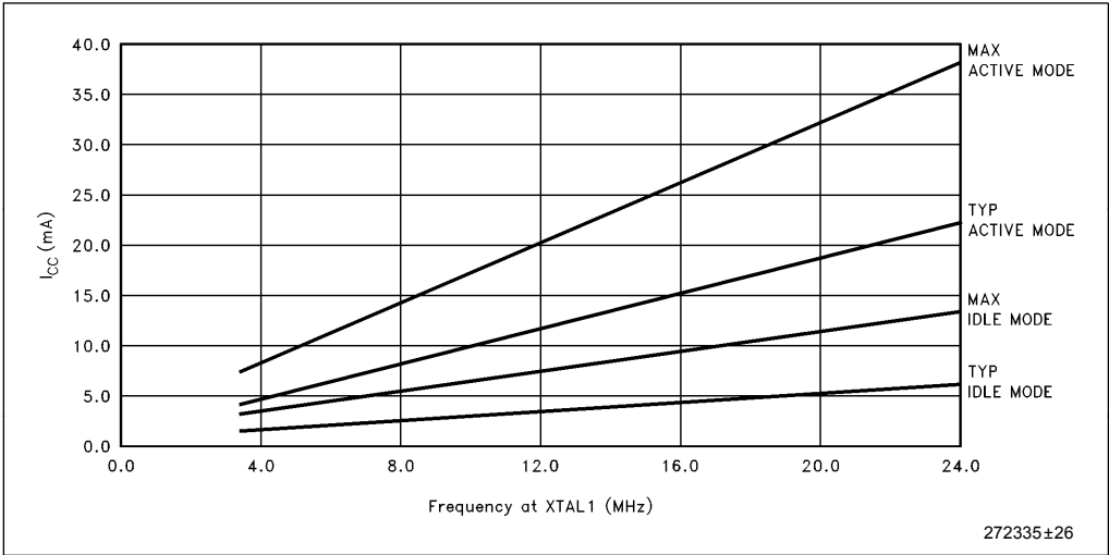
Figure 5. 87C51/BH I_{CC} vs Frequency
