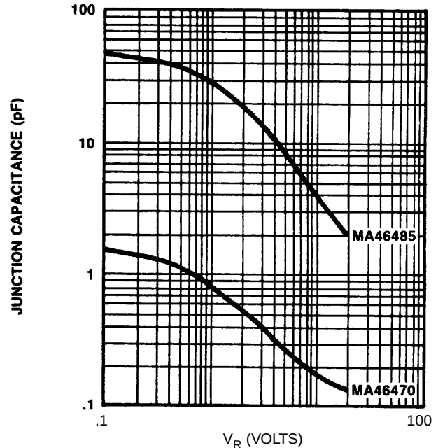
JUNCTION CAPACITANCE vs REVERSE BIAS VOLTAGE ( \gamma = 1.25 ) (CHIPS)
