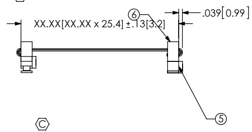
FIG 10 STRAIN RELIEF OPTION (POS 16-25 ONLY) (FFSD-25-D-XX.XX-01-X-N-SR SHOWN) (SAME AS FIG 2, DIFFERENT AS SHOWN) SCALE 1 : 1
