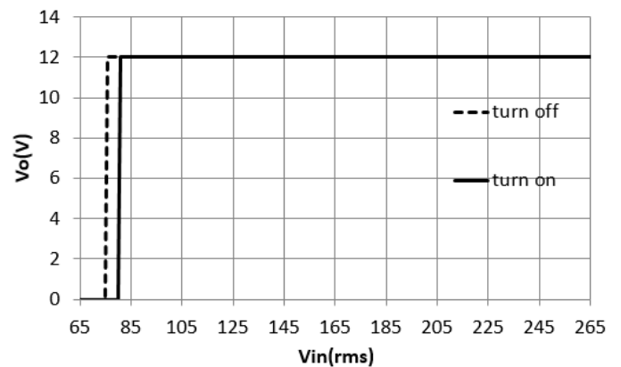
Figure 2: Vout vs. Vin @ Full load
