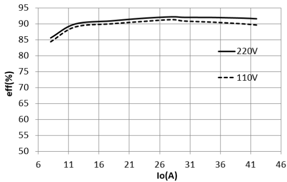
Figure 1: Efficiency vs. Output current @ Vin=110,220VAC
