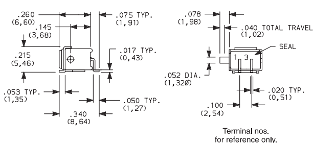
PC MOUNTING
