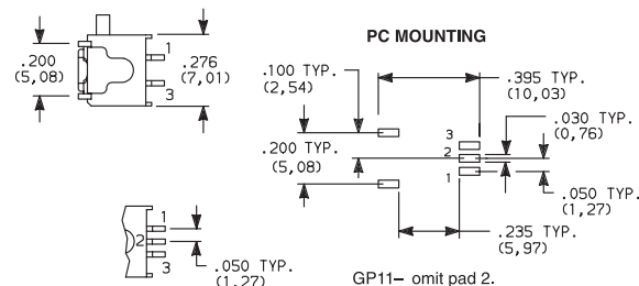
GP12 Model
