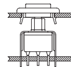
.125" (3,18) PANEL THK.
