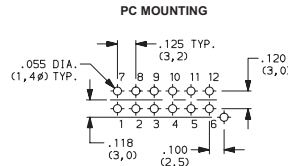
PN41LGS02QE 4PDT
