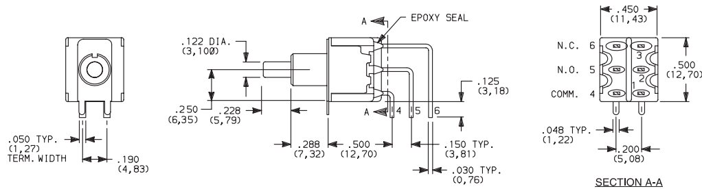
8221SD9AV2GE DPDT
