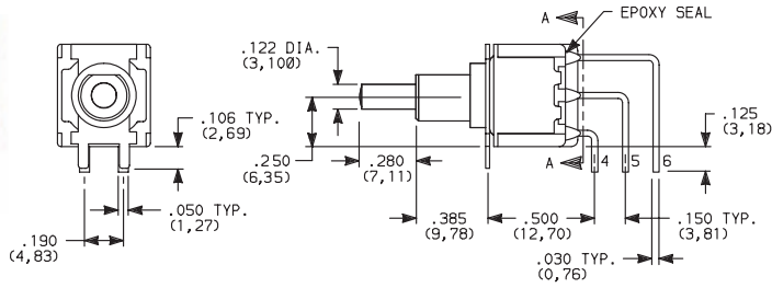
8261SH9AV2BE2 DPDT
