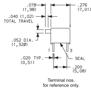
GP11MCBE SPST
