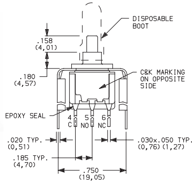
E221SD3V6GE DPDT
