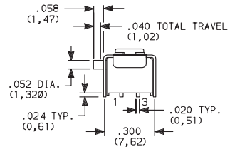
GP11MSV1BE SPST
