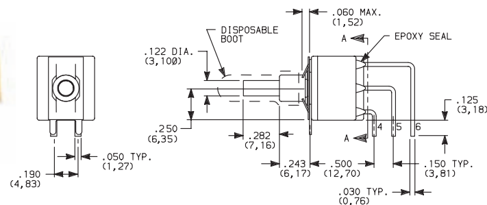
E221SD1AV2GE DPDT
