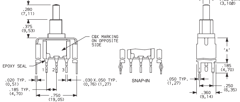
8161SH9_BE2 SPDT
