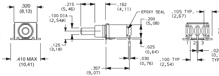
EP12SD1SAPE SPDT
