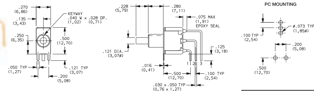
8121SD9AVGE SPDT
