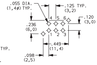
PC MOUNTING
