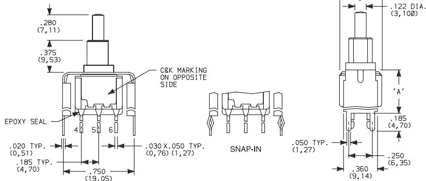
8261SH9_BE2 DPDT
