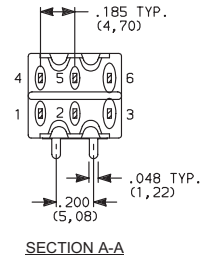
8261SH9ABE2 DPDT
