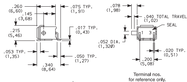
PC MOUNTING
