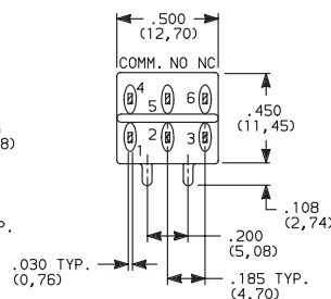
E221SD1AGE DPDT
