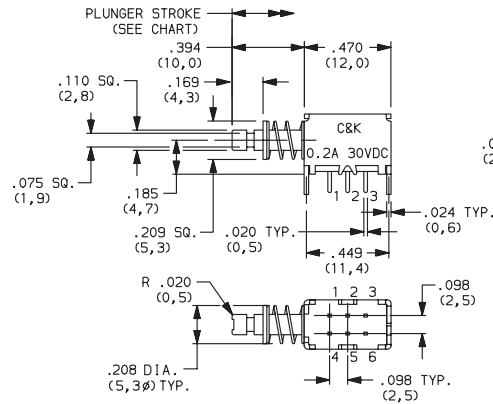
PN21SBSA03QE DPDT
