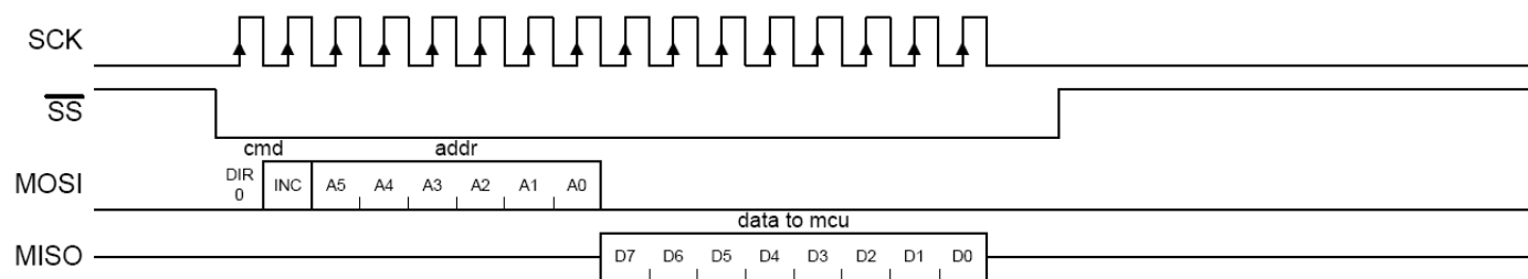
Figure 3 - SPI Single Read Sequence
