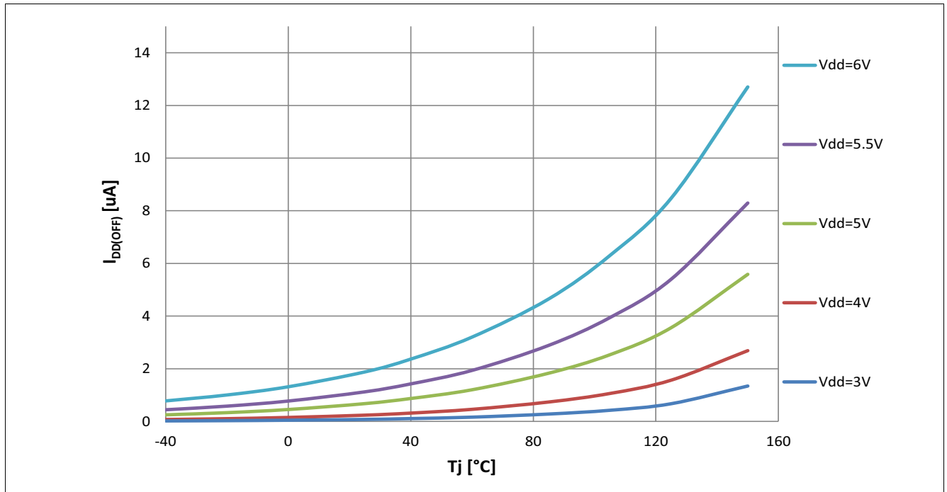
Figure 49 Typical I_{DD(OFF)} vs. T_j @ V_{DD} = 3, 4, 5V , R_{RSP}=0\ \Omega
