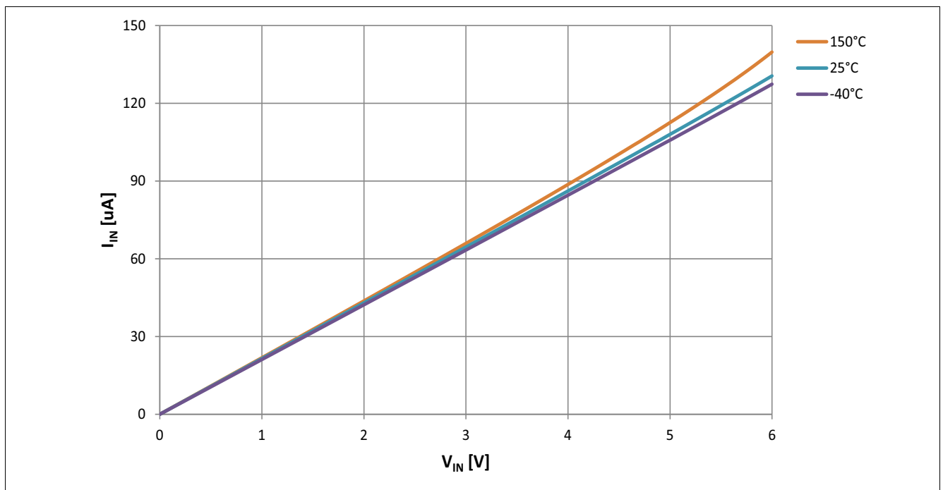
Figure 50 Typical I_{IN} vs. V_{IN} @ T_j = (-40, 25, (85), 150^\circ\text{C})
