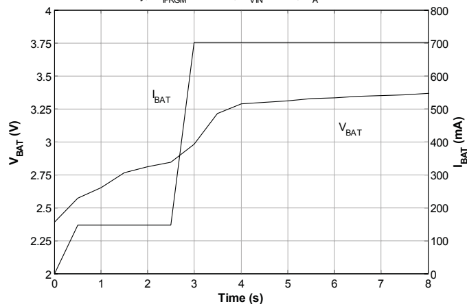
Pre-Charging Battery Voltage and Current
