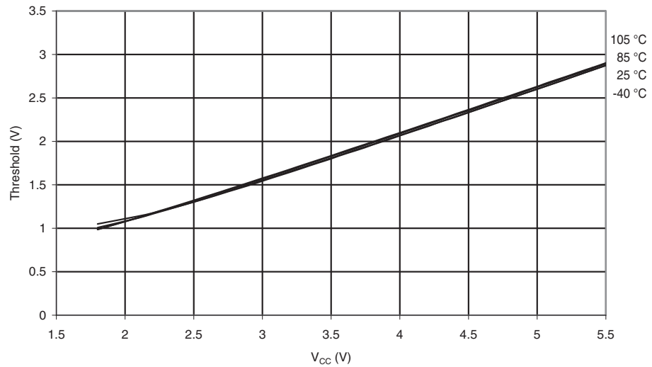
Figure 28-101. ATmega644P: I/O Pin Input Threshold vs. V_{CC} ( V_{IH} , I/O Pin Read as '1').
