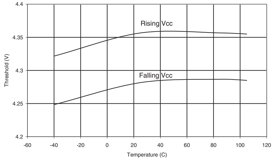
Figure 28-66. ATmega324P: BOD Threshold vs. Temperature ( V_{CC} = 4.3V )
