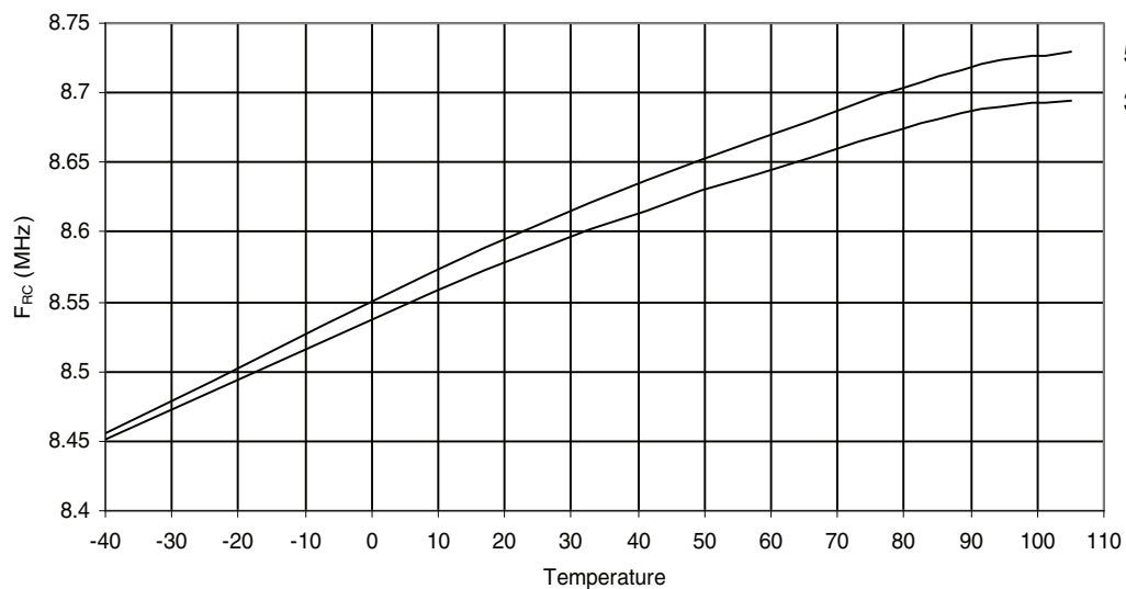
Figure 28-31. ATmega164P: Calibrated 8 MHz RC Oscillator vs. Temperature
