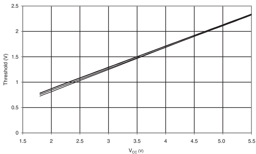
Figure 28-64. ATmega324P: Reset Pin Input Threshold vs. V_{CC} ( V_{IL} , I/O Pin Read as '0')
