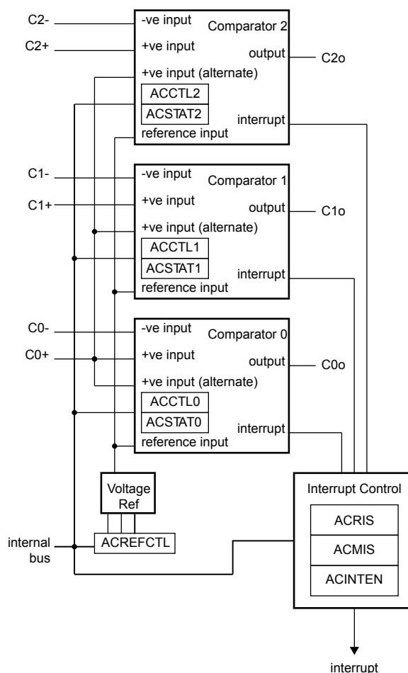
Figure 14-1. Analog Comparator Module Block Diagram
