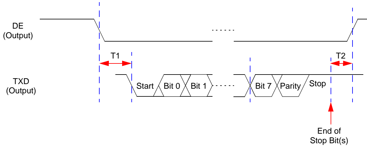
Figure 69. UART Timing without \overline{CTS}
