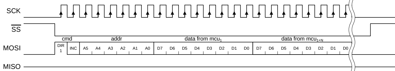
Figure 7. SPI Incrementing Burst Write Sequence
