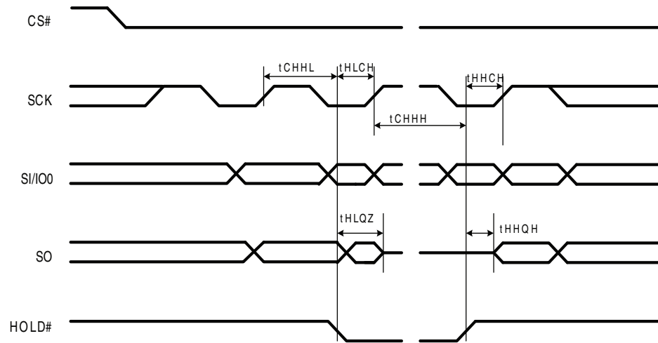
Figure 9.5 Hold Timing
