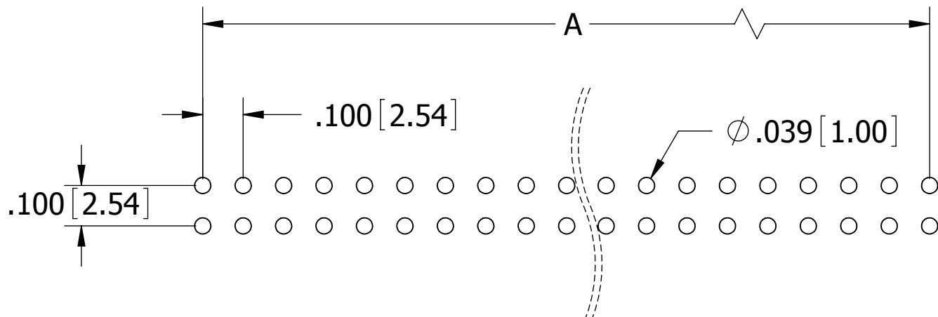
RECOMMENDED PCB HOLE LAYOUT
