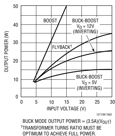
Maximum Output Power
