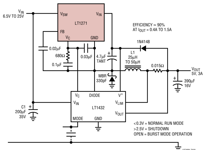
High Efficiency 5V Regulator with Burst Mode™ Operation
