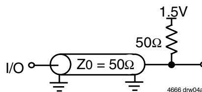
Figure 2b. AC Test Load
