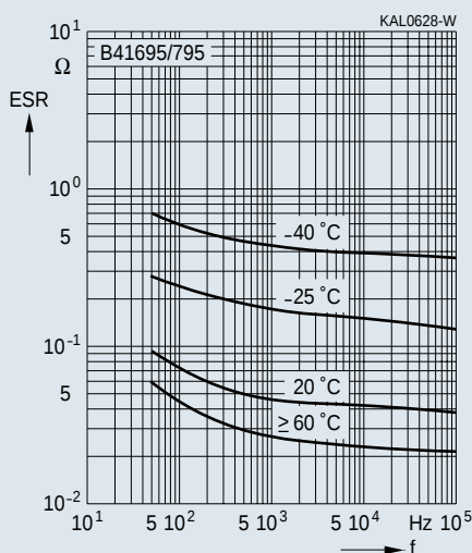
Equivalent series resistance ESR versus frequency at different temperatures Typical behavior for 2200 \mu F/40 V
