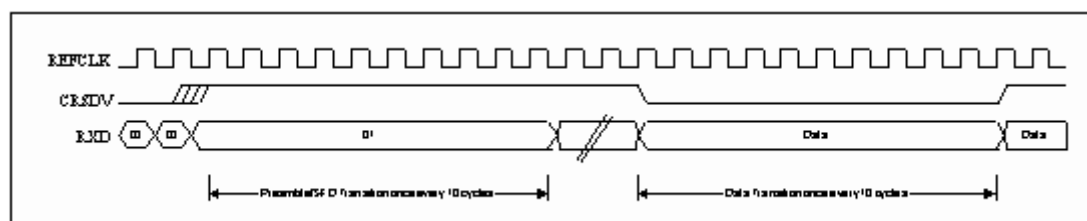
Figure 9 10M RMI Receive Diagram
