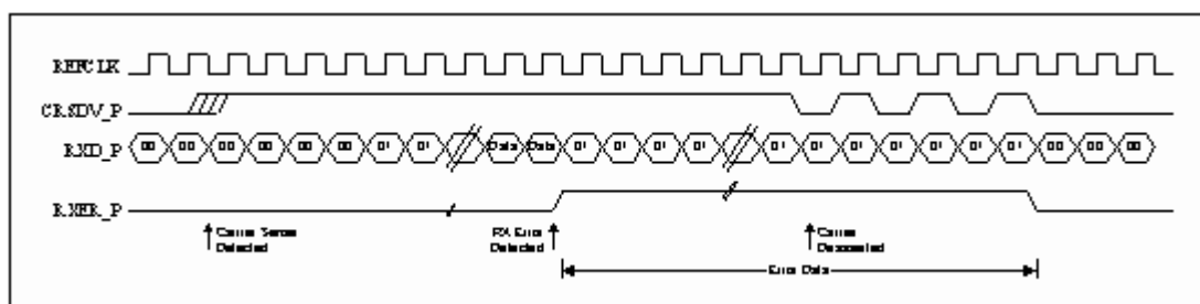
Figure 8 RMI Reception with Symbol Error
