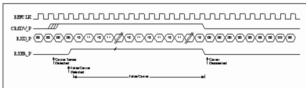
Figure 7 RMI Reception with False Carrier (100M Only)
