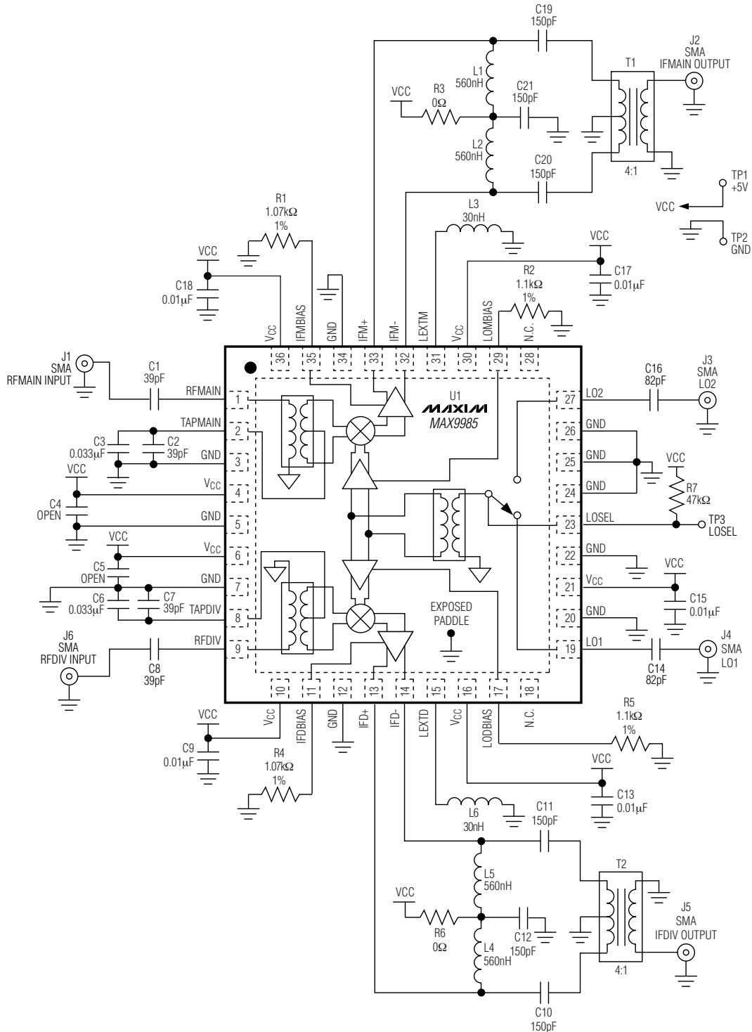
Figure 2. MAX9985 EV Kit Schematic
