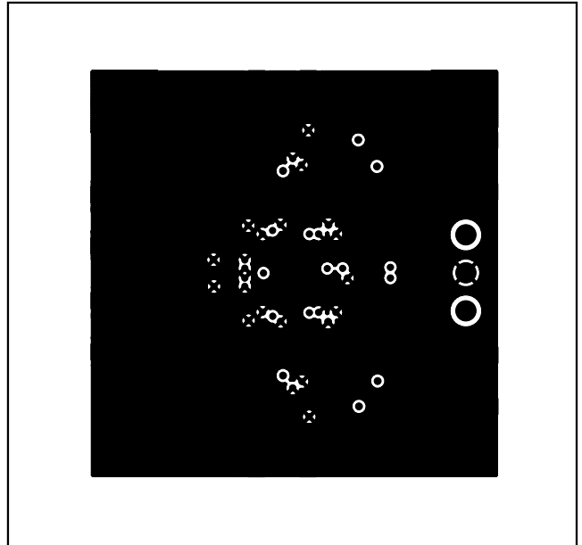
Figure 8. MAX9985 EV Kit PCB Layout—Bottom Layer Metal
